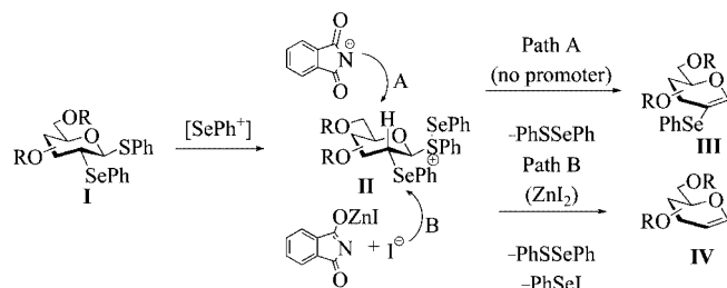
Scheme 3. Plausible mechanism for the observed product distribution during the cyclization of 3,4- O -isopropylidene-protected alkyl sulfides induced by electrophilic selenium species.
