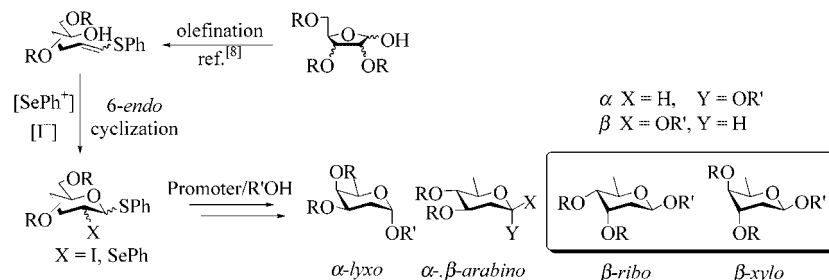
Scheme 1. Stereoselective synthesis of 2-deoxy- and 2,6-dideoxyglycosides of D- lyxo , D- arabino , D- ribo and D- xylo configurations through an olefination–cyclization–glycosylation sequence.
